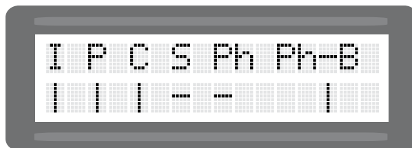
STOP button and photocell are triggered. All other inputs are okay.
