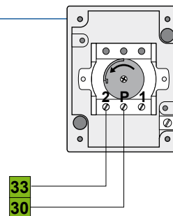
CLOSE-button (e.g. key switch EPZ 1-2T)
