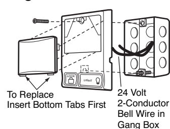
Figure 4 REMOVE COVER
