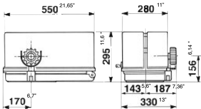
Abmessungen in mm/inch
