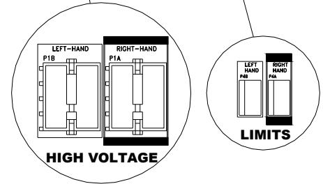
Figure 17: Control Board Settings for LH/RH Operation
