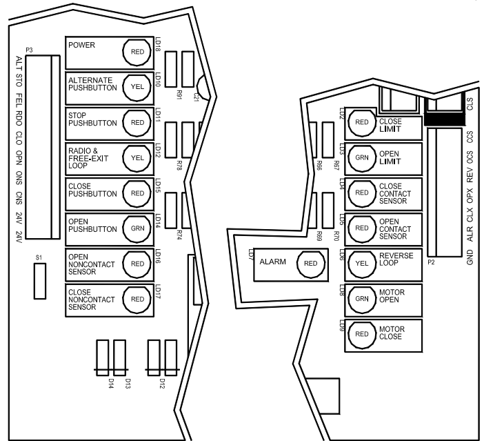
Figure 22: Indicator Lamps
