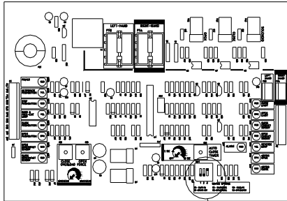
LOCATION OF SWITCH SELECTABLE OPTIONS
