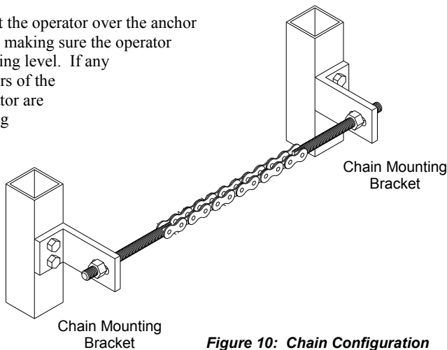
Figure 10: Chain Configuration
