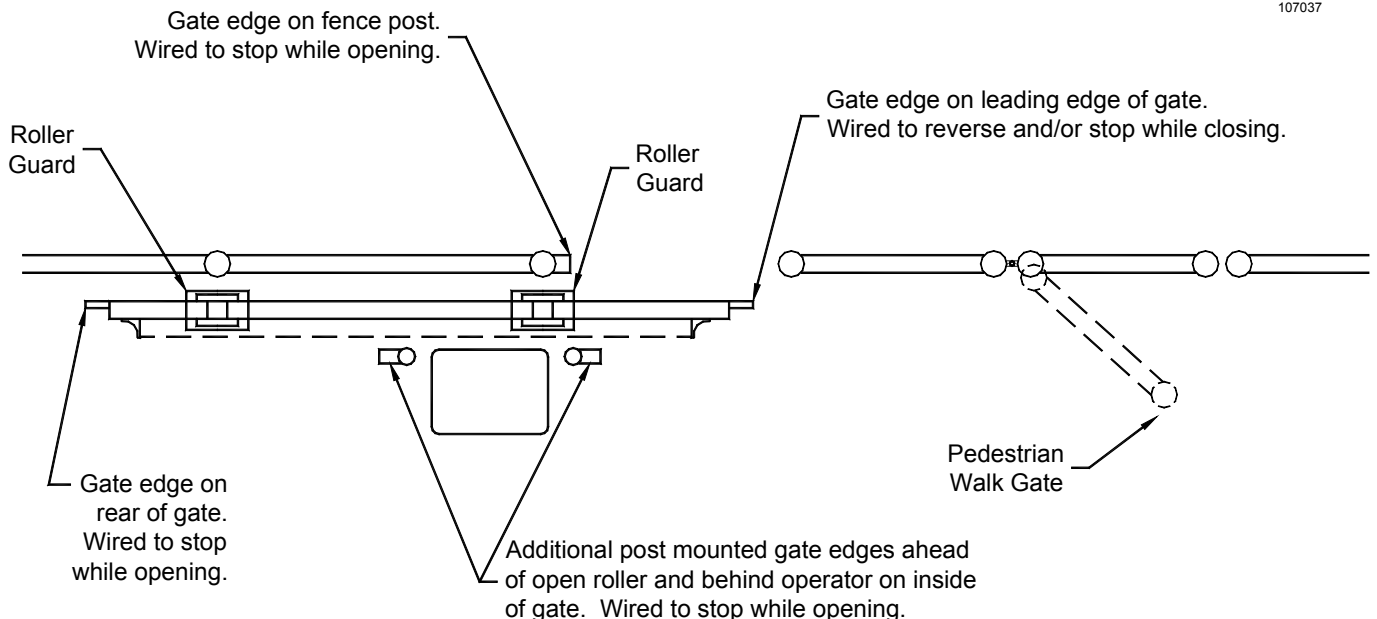
Figure 25: Entrapment Protection
