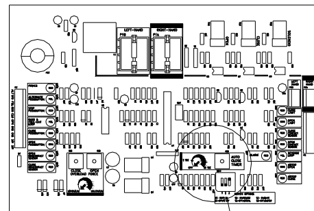
LOCATION OF AUTOCLOSE TIMER ADJUSTMENT
