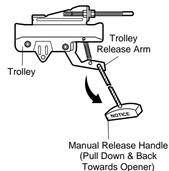
Lockout position
