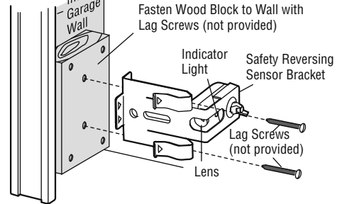
Figure 2 WALL MOUNT (RIGHT SIDE)
