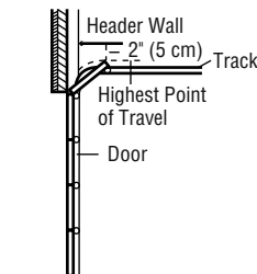
Sectional door with curved track
