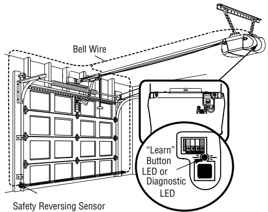
Safety Reversing Sensor
