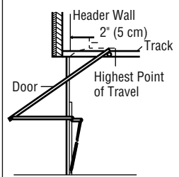
One-piece door with horizontal track
