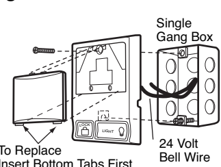
Figure 4 REMOVE COVER
