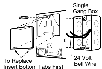
Figure 4 REMOVE COVER
