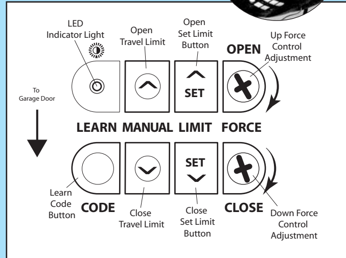
FIG. 6-1 Limit controls.
