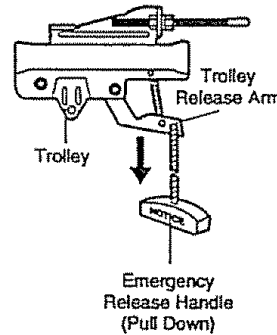
Manual disconnect position
