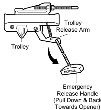
Lockout position
