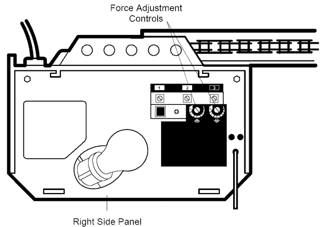
Right Side Panel
