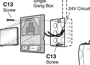
Multi-Function Door Control: Gang Box Installation
