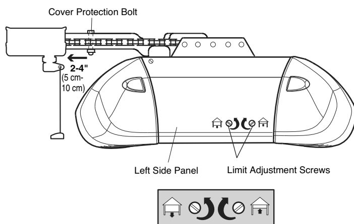
ADJUSTMENT LABEL
