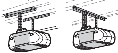
Finished Ceiling
