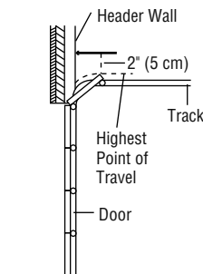
Sectional door with curved track
