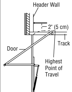
One-piece door with horizontal track
