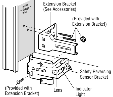
Figure 3 WALL MOUNT (RIGHT SIDE)
