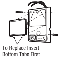
Figure 3 MULTI-FUNCTION DOOR CONTROL (BACK)
