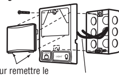
Figure 2 INSTALLATION PRÉ-CÂBLÉE
