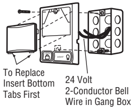
Figure 4 REMOVE COVER
