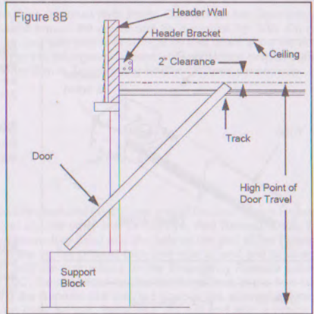
One-Piece Door with Horizontal Track
