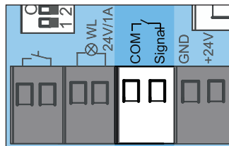
Fig. Terminal block for a 2-wire photocell
