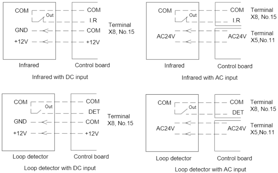
Schematic diagram
